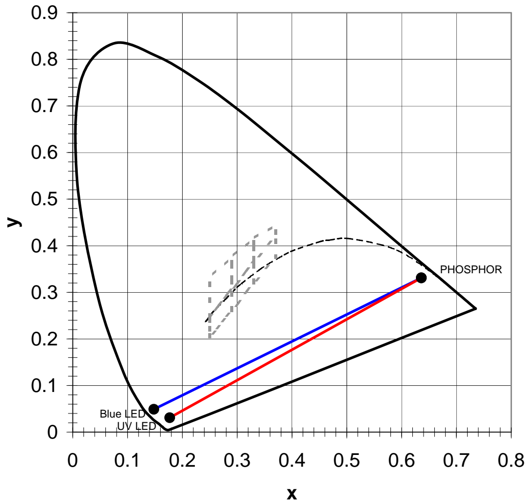
CIE Chart
