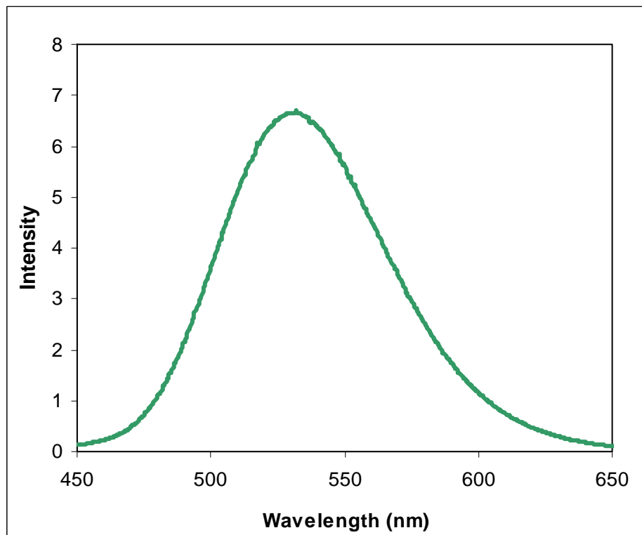
Emission Spectrum
