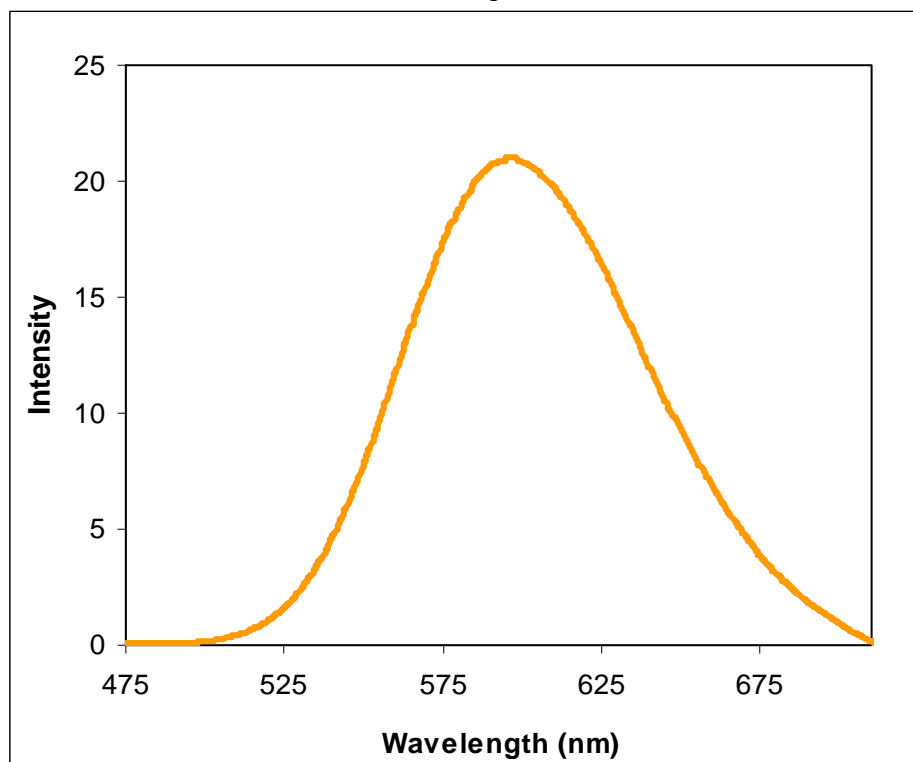
Emission Spectrum
