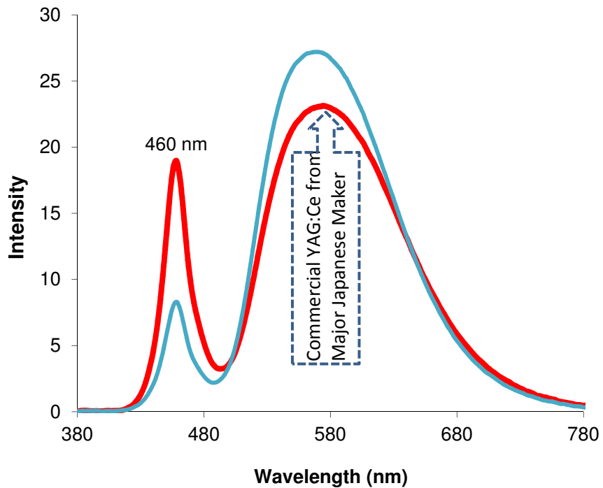
Relative Emission using Blue LED Excitation (Reflection Mode)
